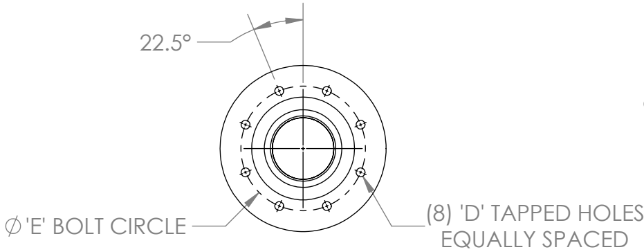
4" SUCTION FLANGE DETAIL ANSI 150# ANSI 300# ISO/DIN PN40
