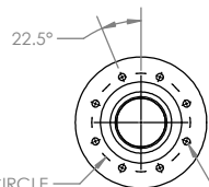
4" SUCTION FLANGE DETAIL ANSI 150# ANSI 300# ISO/DIN PN40
