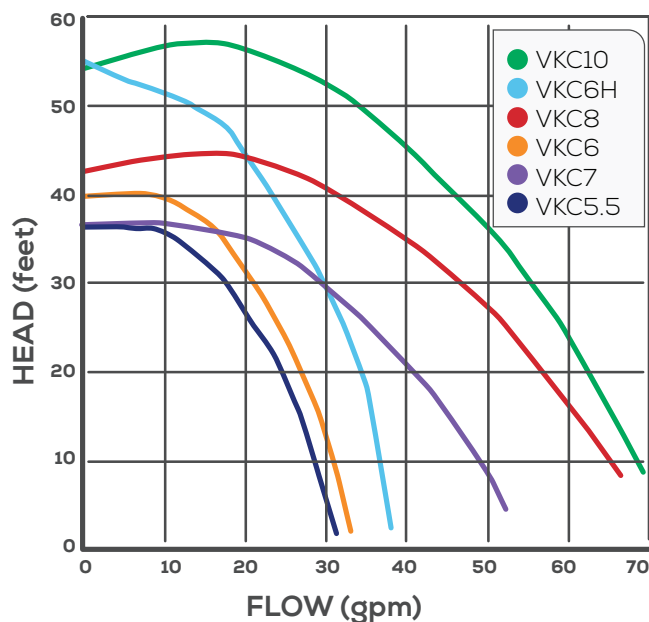
60 Hz, 3450 rpm
