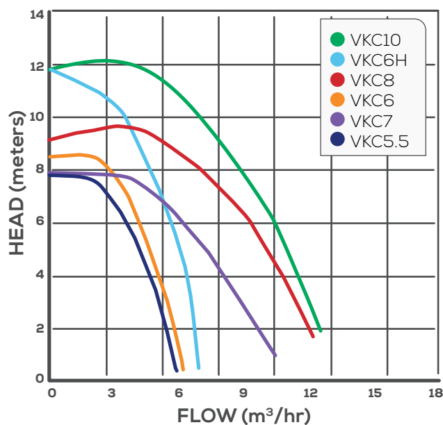
50 Hz 2900 rpm
